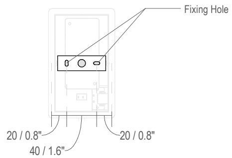
Fixing Dimensions
