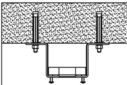
CEILING-MOUNT BRACKET
