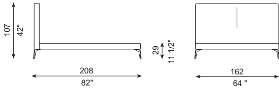
REF. 648-CM1 Colchón - Mattress 150 cm x 190 cm
