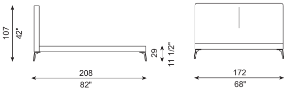
REF. 648-CM3 Colchón - Mattress 160 cm x 190 cm
