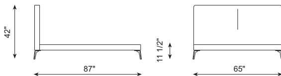
REF. 648-QUEEN SIZE Colchón - Mattress 153x203 / 60 1/4" x 80"
