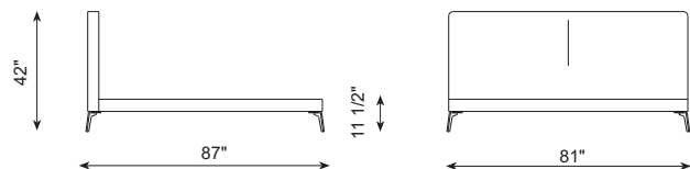
REF. 648-KING SIZE Colchón - Mattress 193x203 / 76" x 80"
