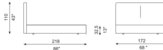
REF. 652-CM4 Colchón - Mattress 160 cm x 200 cm
