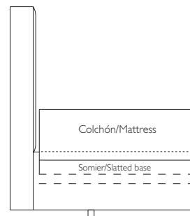
REF. 652-KING SIZE Colchón - Mattress 193x203 / 76" x 80"
