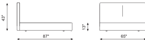
REF. 652-QUEEN SIZE Colchón - Mattress 153x203 / 60 1/4" x 80"
