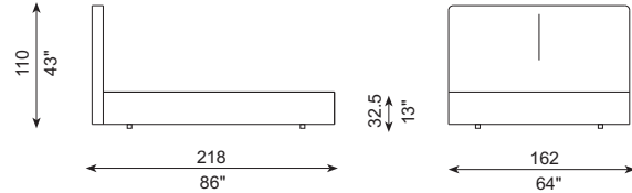
REF. 652-CM2 Colchón - Mattress 150 cm x 200 cm
