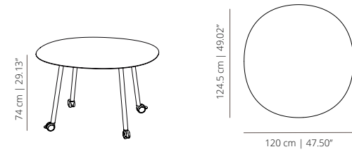
MAAD120 table 120 | 47 1 / 4 with casters
