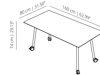
MAA160_ table 160x80 | 31 1 / 2 x 62 63 / 64 with casters
