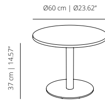
ST37D60_ table round 60 | table round 23 5/8
