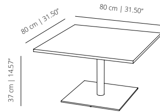
ST37C80_ table 80x80 | table 31 1/2 x 31 1/2
