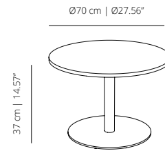
ST37D70_ table round 70 | table round 27 6/16
