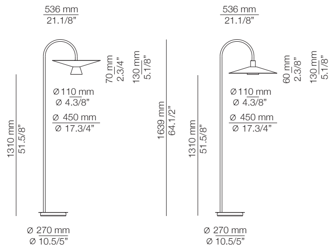
BEL_4149LG: with large metall shade Ø 450mm + glass shade
