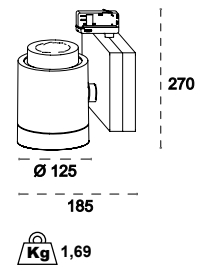
CYLINDER LED
