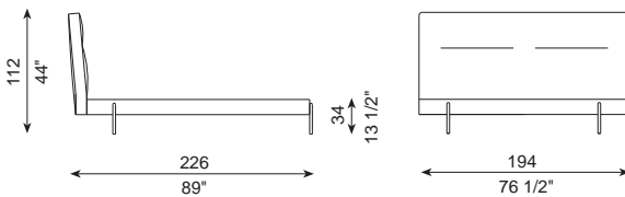
REF 616-CM5 Colchón - Mattress 180 cm x 200 cm
