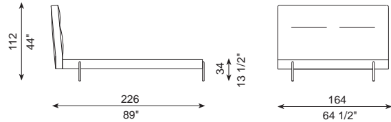
REF 616-CM2 Colchón - Mattress 150 cm x 200 cm
