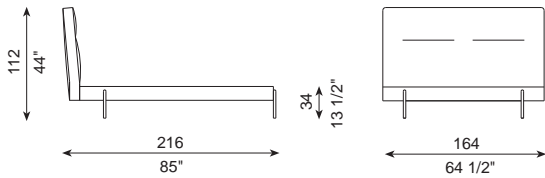
REF 616-CM1 Colchón - Mattress 150 cm x 190 cm
