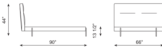
REF 616-QUEEN SIZE Colchón - Mattress 153x203 / 60 1/4" x 80"
