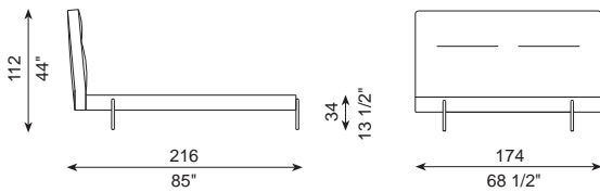
REF 616-CM3 Colchón - Mattress 160 cm x 190 cm
