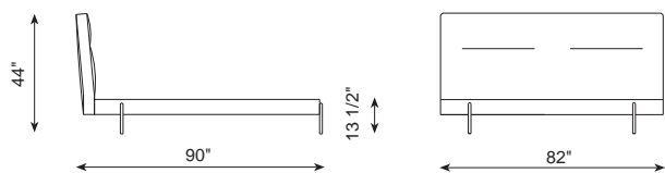
REF 616-KING SIZE Colchón - Mattress 193x203 / 76" x 80"
