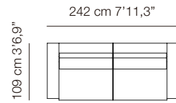
Sofá 4 plazas_ Ref. 108240
