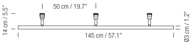
(2) Structure for three lampshade
