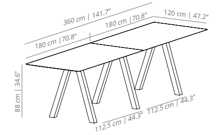
TRMEDCNEX Double table 360 x 120 | 78.7 x 47.2"
