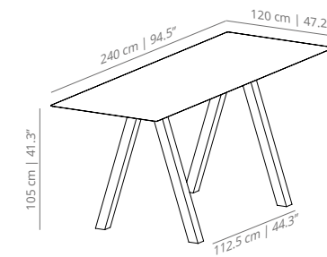
TRMESACNEX table 240 x 120 | 94.5" x 47.2"
